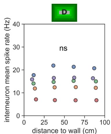
Fig. S10. Interneuron firing rate is constant at all distances to walls. Mean spike rate of all interneurons detected in each animal at different distances to wall in environment D.
