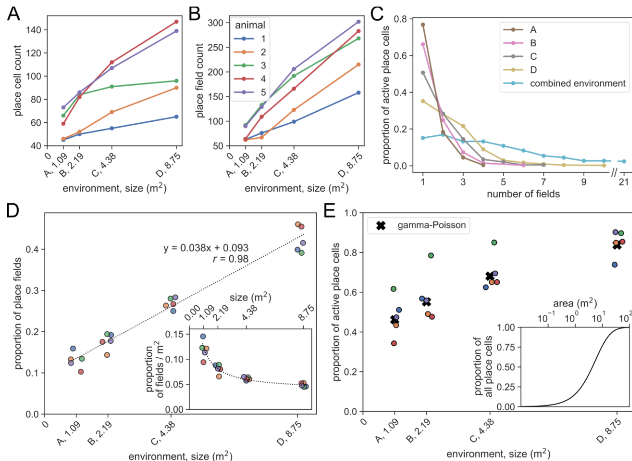
Fig. 2. Place cells are more likely to be active and have more fields in large environments. Number of active place cells (A) and place fields (B) by environment area. (C) Distribution of place field counts per cell by environment. Only cells with at least one field in any environment are included. (D) Larger environments had more place fields, here shown as a proportion of all fields detected in each animal across the four environments (Kruskal-Wallis: H = 17.6 , p = 5.36 \times 10^{-4} , N = 5 ), scaling linearly with environment area (dashed line, linear regression fit, r = 0.982 , p = 10^{-14} , N = 20 ). Inset shows place field count by environment area, regression line shown with same parameters as main plot (Kruskal-Wallis: H = 17.9 , p = 4.71 \times 10^{-4} , N = 5 ). Animal colors same as B, points jittered to facilitate visualisation. (E) The proportion of all recorded place cells that were recruited
