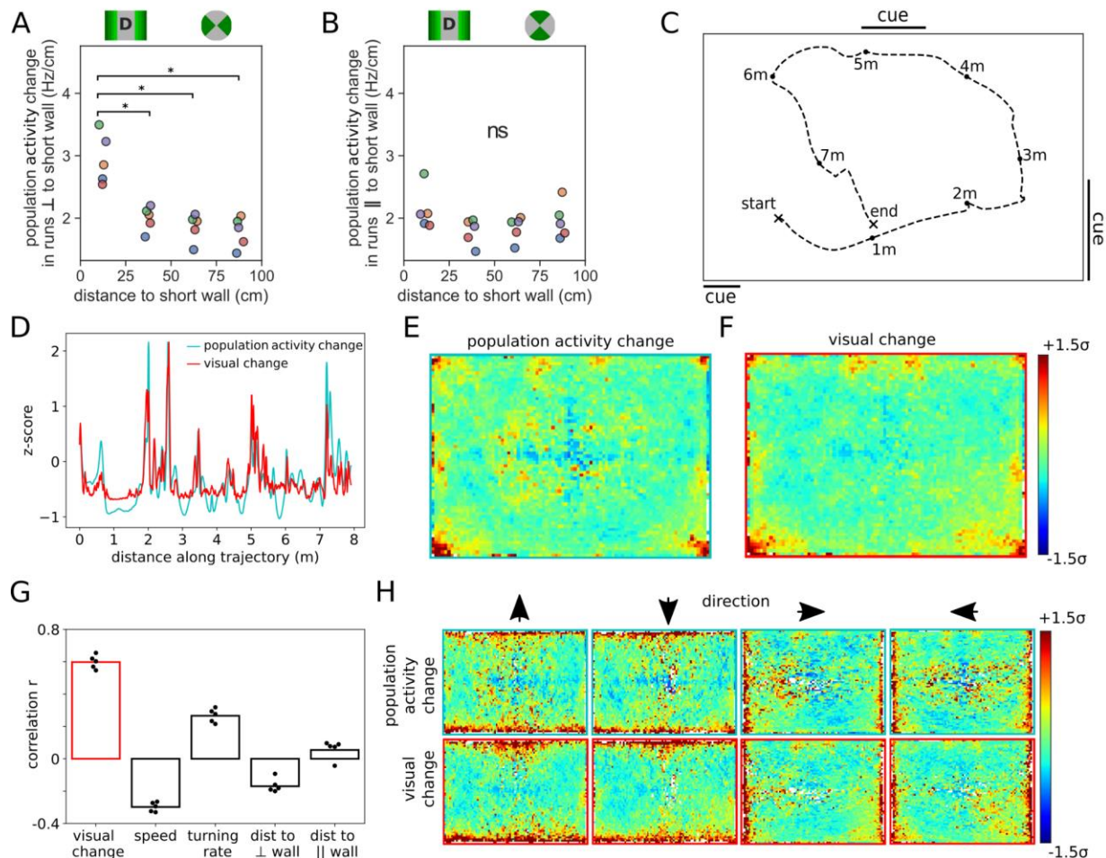
Fig. 4. The rate of change in the place cell population mirrors the rate of change in the visual scene.
