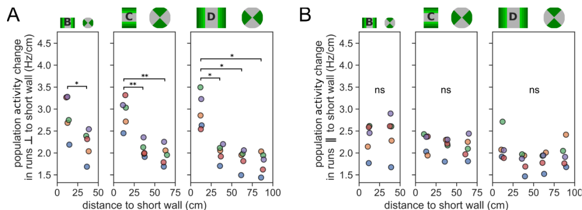
Fig. S11. Population activity change was higher in runs orthogonal and close to walls in all environments. (A) Euclidean distance between vectors representing population activity at different distances to the short walls of each environment, only including runs orthogonal to the short wall. Pair-wise post hoc tests adjusted for multiple comparisons using Benjamini/Hochberg (non-negative) correction. (B) Same as A , but runs parallel to the short wall.
